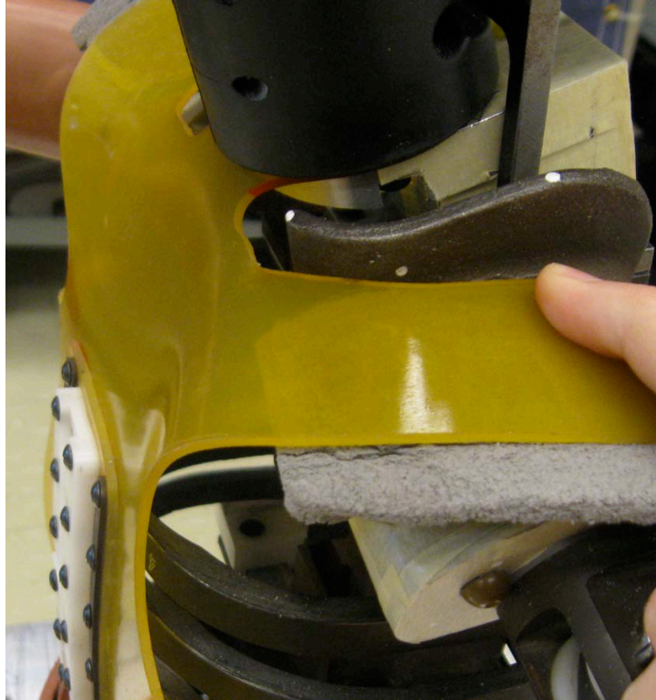
Figure 16. Bib assembly fit on ATD shoulder with clavicle link rotated down and clavicle rotated rearward.
