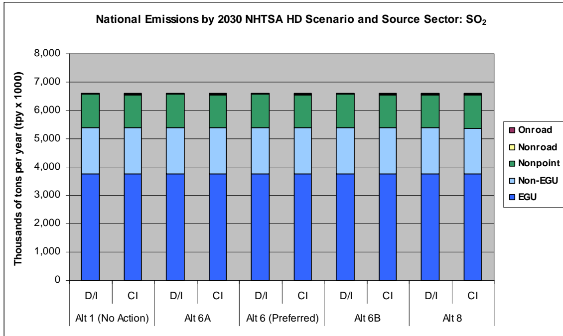
Figure 2.3-3c. National Emissions Totals for SO 2 for 2030 for the HD Alternatives
