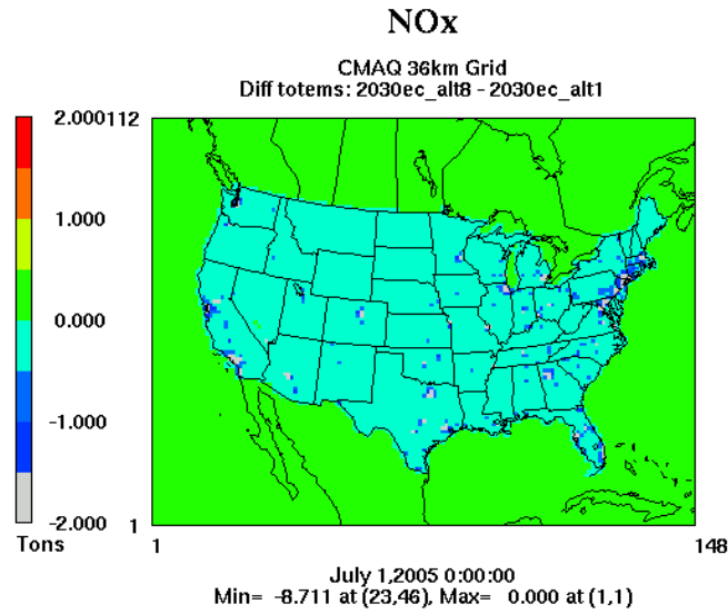
Figure 2.3-2b. Difference in Daily NO x Emissions for 1 July 2030 for Alternative 8 Minus the No Action Alternative Under the Direct and Indirect Effects Scenario
