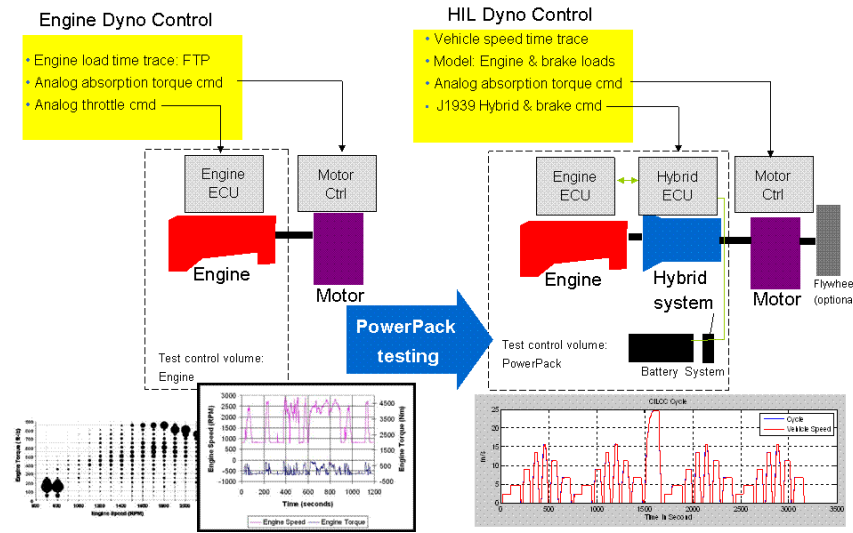
Figure 3-5 Hardware-in-the-Loop Post-Transmission Powerpack Test Configuration
