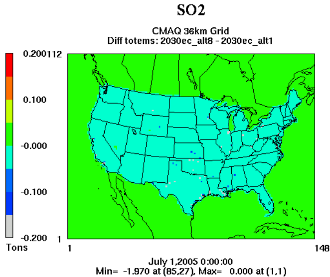
Figure 2.3-2c. Difference in Daily SO 2 Emissions for 1 July 2030 for Alternative 8 Minus the No Action Alternative Under the Direct and Indirect Effects Scenario
