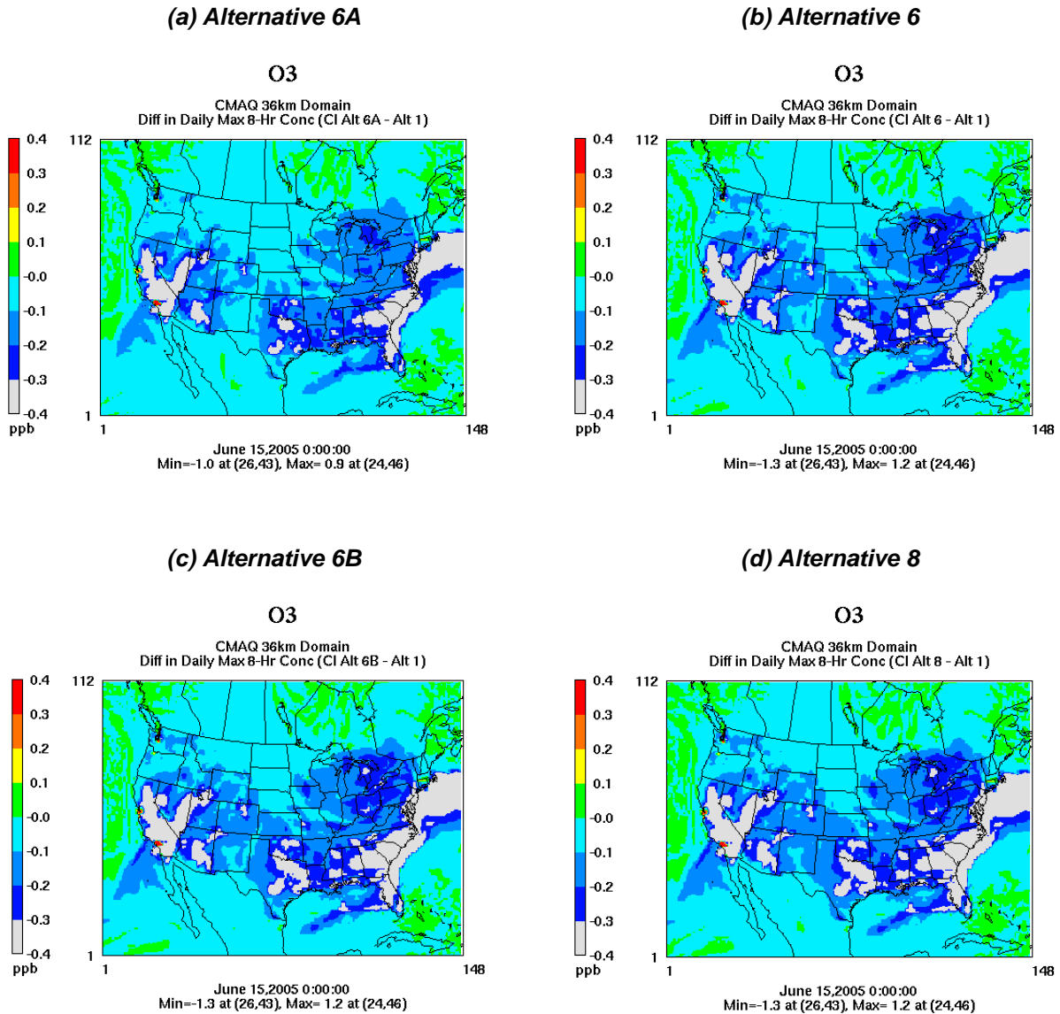
Figure 3.3.2-2. Difference in Simulated Daily Maximum 8-Hour Ozone Concentration (ppb) for 15 June Alternatives 6A, 6, 6B and 8 Minus the No Action Alternative Under the Cumulative Impacts Scenario
