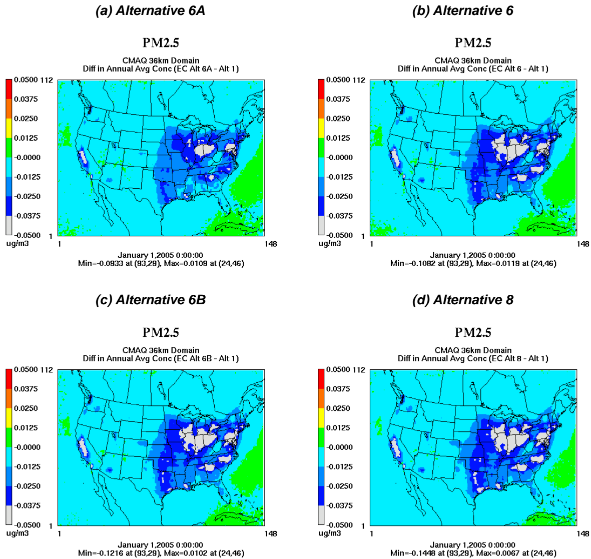
Figure 3.3.1-5. Difference in Annual Average PM 2.5 Concentration ( \mu\text{g}\text{m}^{-3} ): Alternatives 6A, 6, 6B and 8 Minus the No Action Alternative Under the Direct and Indirect Effects Scenario
