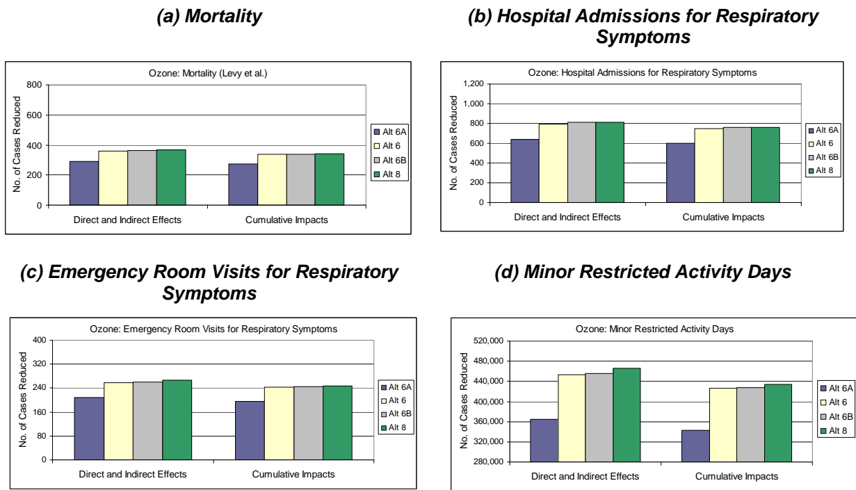
Figure 4.3.3-1a. BenMAP-Derived Changes in Selected Health Outcomes for the Direct and Indirect Effects and Cumulative Impacts Scenarios: Ozone
