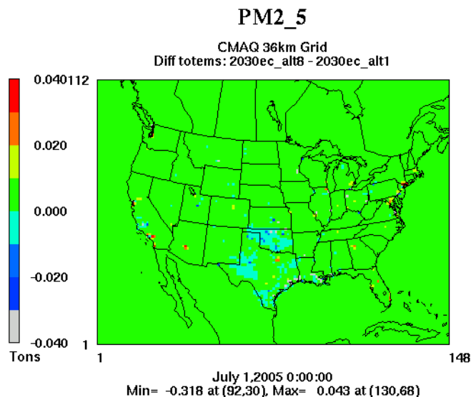
Figure 2.3-2d. Difference in Daily PM 2.5 Emissions for 1 July 2030 for Alternative 8 Minus the No Action Alternative Under the Direct and Indirect Effects Scenario
