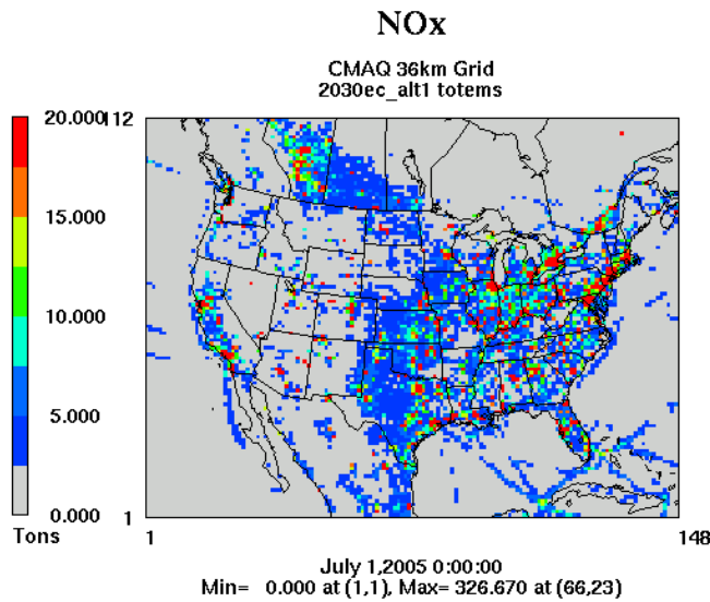
Figure 2.3-1b. Daily NO x Emissions for 1 July 2030: No Action Alternative Under the Direct and Indirect Effects Scenario
