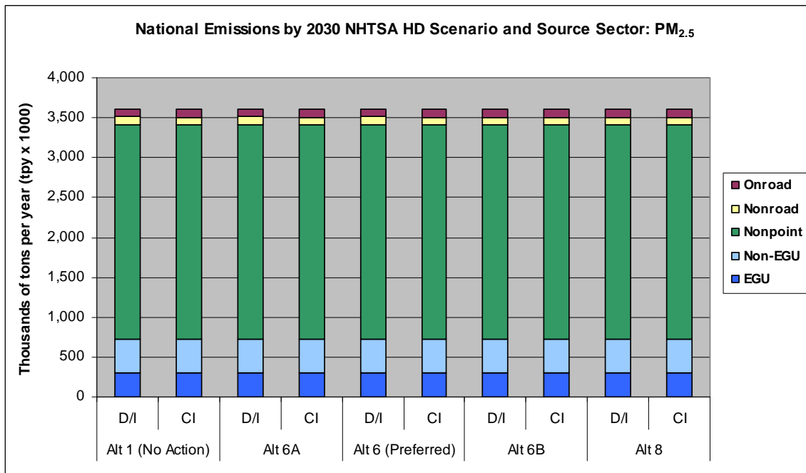
Figure 2.3-3d. National Emissions Totals for PM 2.5 for 2030 for the HD Alternatives
