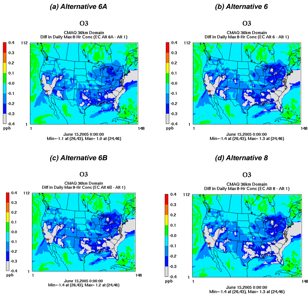
Figure 3.3.1-2. Difference in Simulated Daily Maximum 8-Hour Ozone Concentration (ppb) for 15 June: Alternatives 6A, 6, 6B and 8 Minus the No Action Alternative Under the Direct and Indirect Effects Scenario
