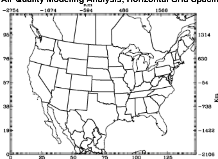
Figure 1.2-1. CMAQ Modeling Domain for the NHTSA HD Fuel Efficiency Improvement Program Air Quality Modeling Analysis; Horizontal Grid Spacing is 36 km
