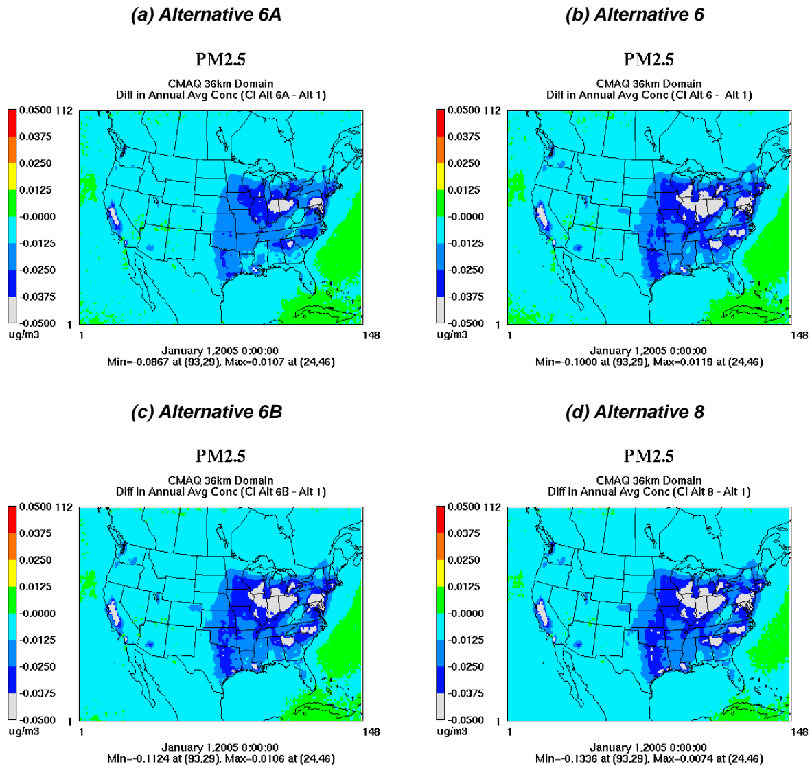
Figure 3.3.2-4. Difference in Annual Average PM 2.5 Concentration ( \mu\text{g}\text{m}^{-3} ): Alternatives 6A, 6, 6B and 8 Minus the No Action Alternative Under the Cumulative Impacts Scenario
