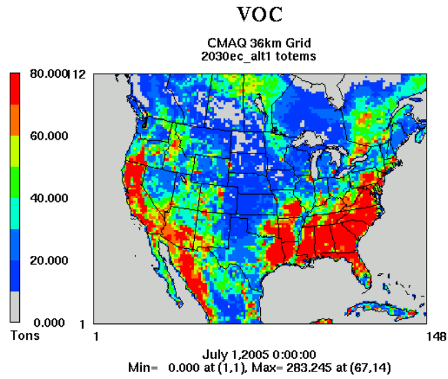
Figure 2.3-1a. Daily VOC Emissions for 1 July 2030: No Action Alternative Under the Direct and Indirect Effects Scenario
