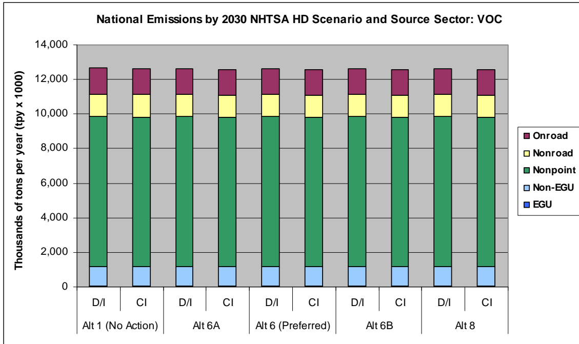
Figure 2.3-3a. National Emissions Totals for VOC for 2030 for the HD Alternatives
