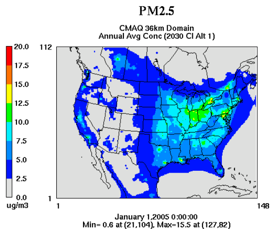
Figure 3.3.2-3. Simulated Annual Average PM 2.5 Concentration ( \mu\text{g}\text{m}^{-3} ) for 2030: No Action Alternative Under the Cumulative Impacts Scenario
