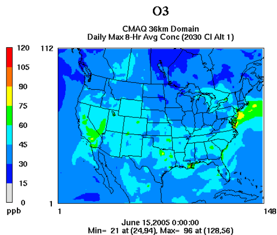
Figure 3.3.2-1. Simulated Daily Maximum 8-Hour Ozone Concentration (ppb) for 15 June 2030: No Action Alternative Under the Cumulative Impacts Scenario
