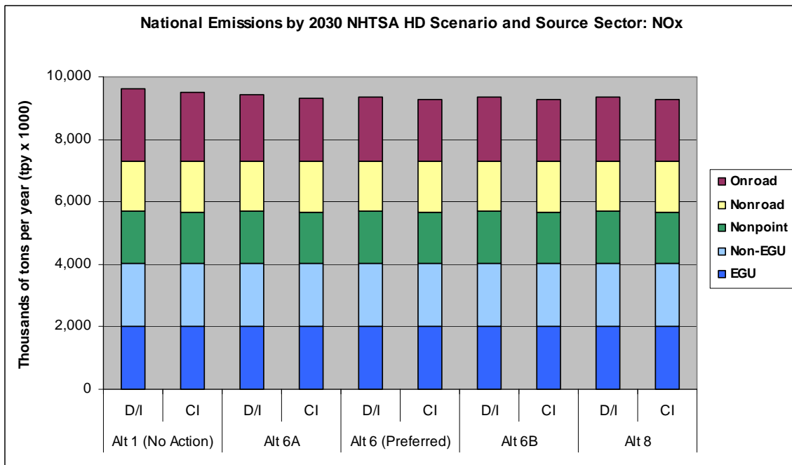
Figure 2.3-3b. National Emissions Totals for NO x for 2030 for the HD Alternatives
