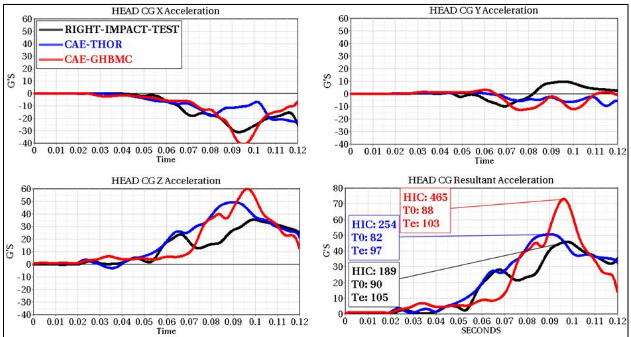
Figure 89: Passenger Head CG Acceleration
