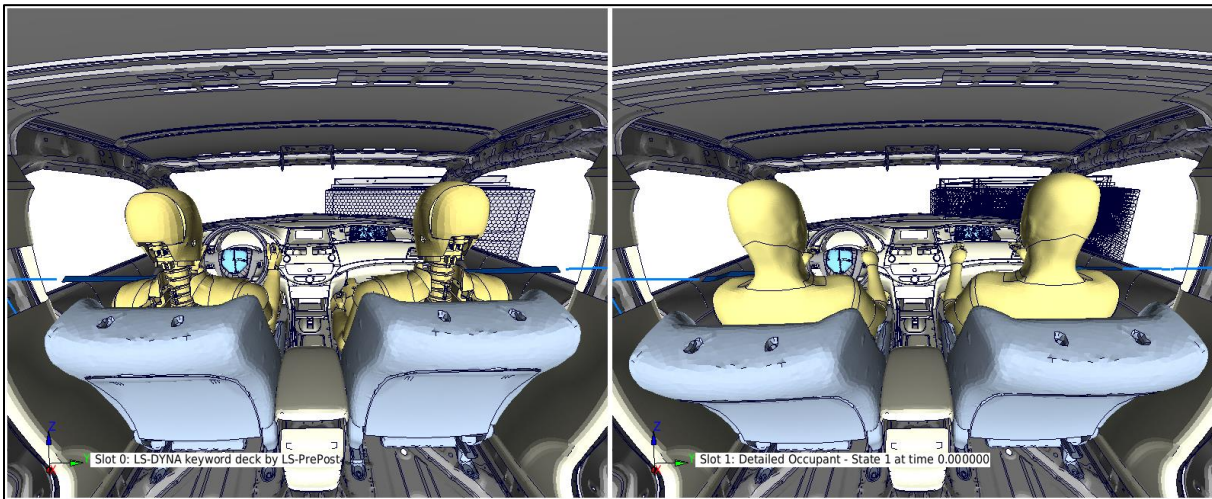
Figure 83: THOR CAE Versus GHBM Model at 0 ms
