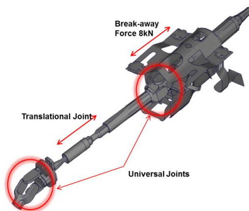
Figure 19: Steering Column Joints
