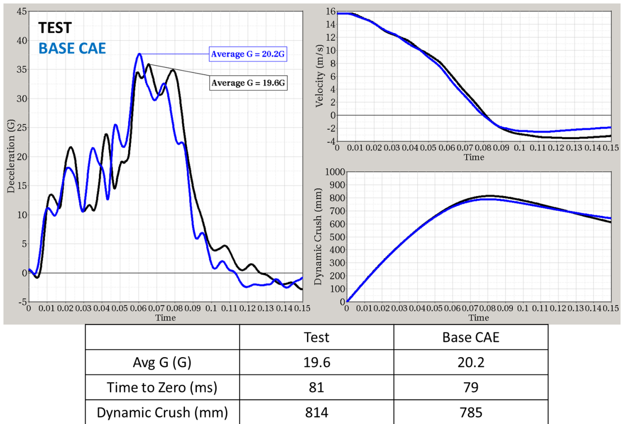
Figure 4: Test Versus Baseline – Vehicle Motion Comparison
