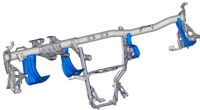
Figure 21: Instrument Panel Structure With Knee Bolsters (Blue)
