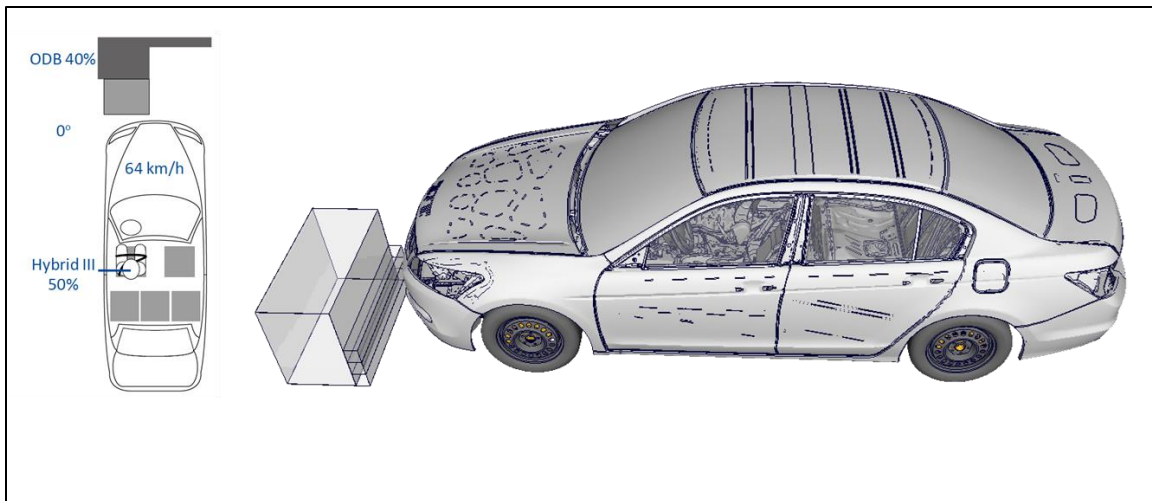
Figure 5: IIHS Frontal Moderate - Test and LS-DYNA Model Setup
