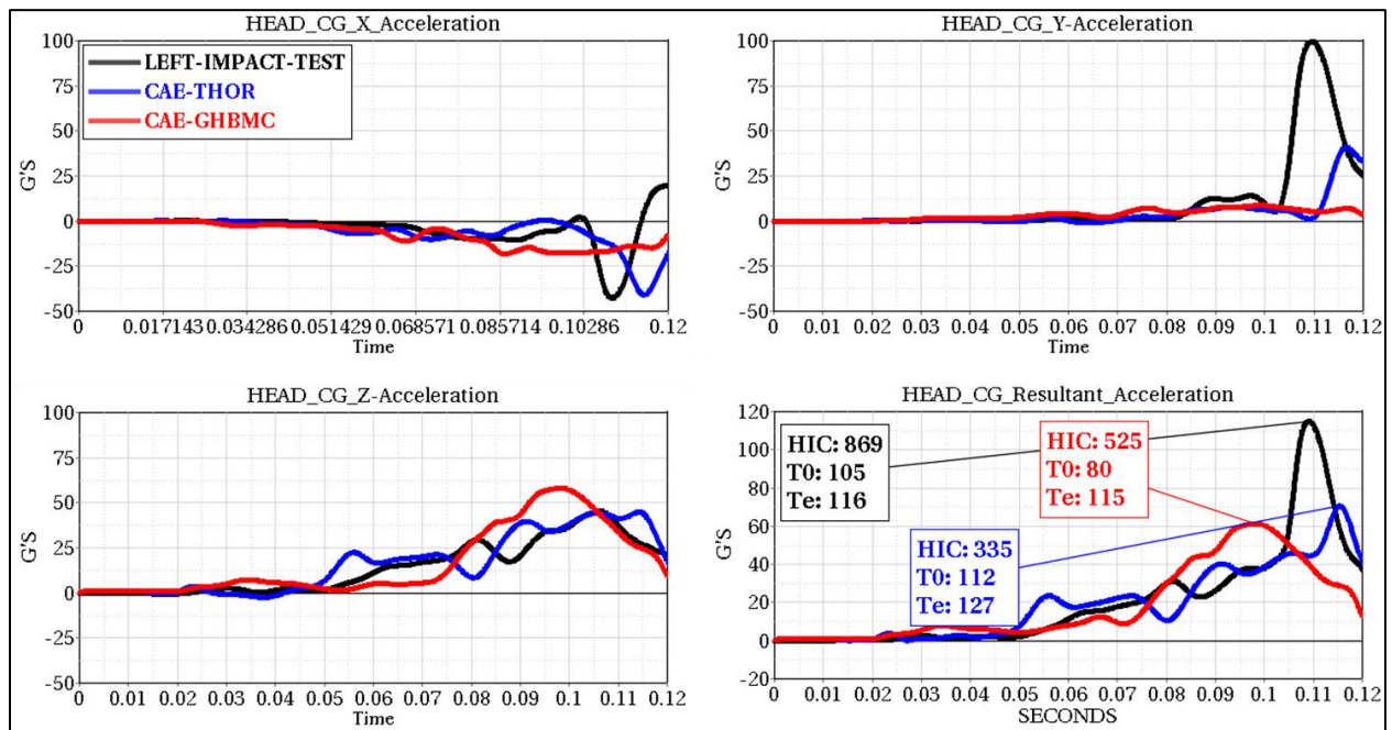
Figure 78: Passenger Head CG Acceleration
