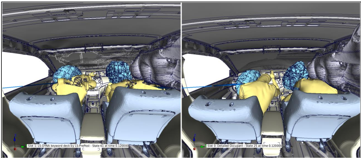
Figure 87: THOR CAE Versus GHBM Model at 120 ms
