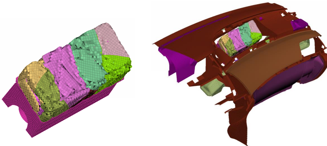
Figure 32: Folded Passenger Air Bag
