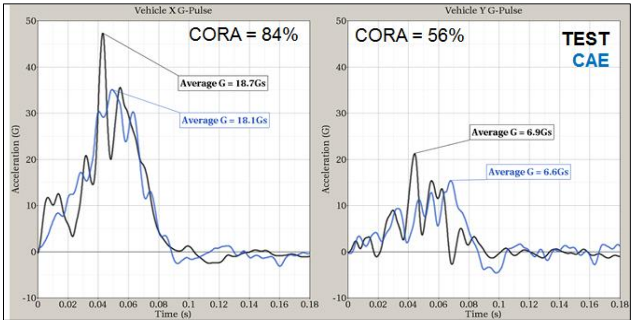
Figure 15: Test Versus CAE X and Y Acceleration Pulse
