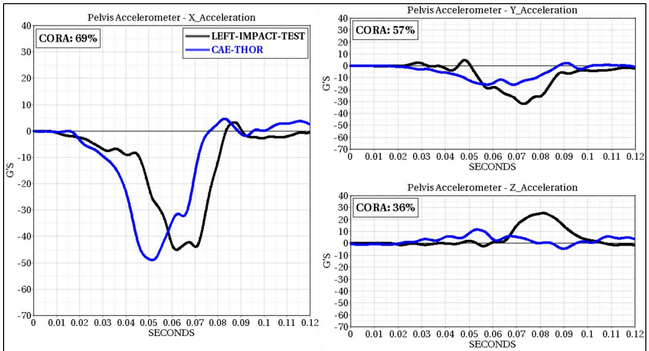
Figure 54: Driver Pelvic CG Acceleration
