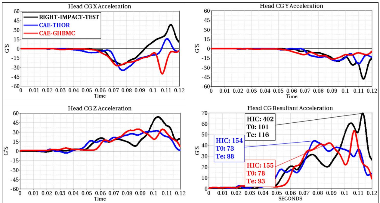
Figure 88: Driver Head CG Acceleration
