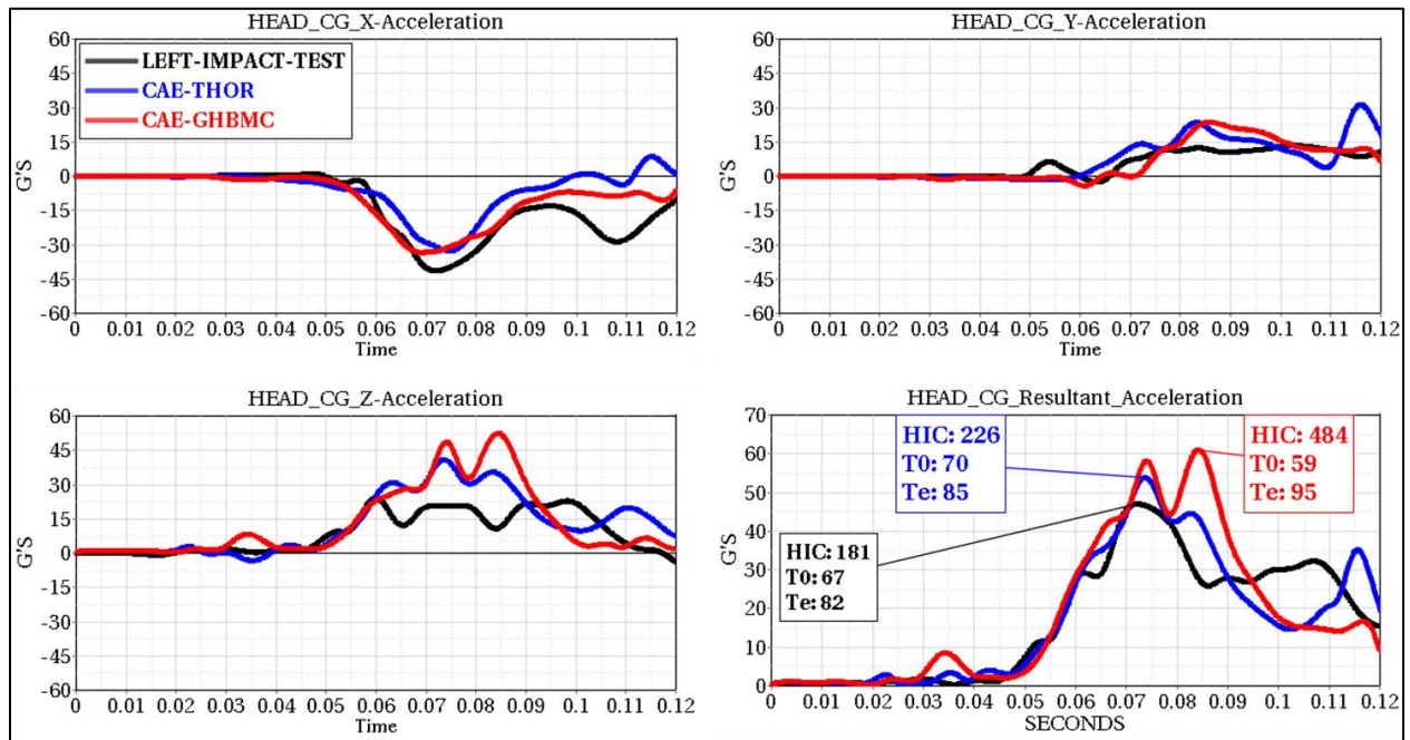
Figure 77: Driver Head CG Acceleration
