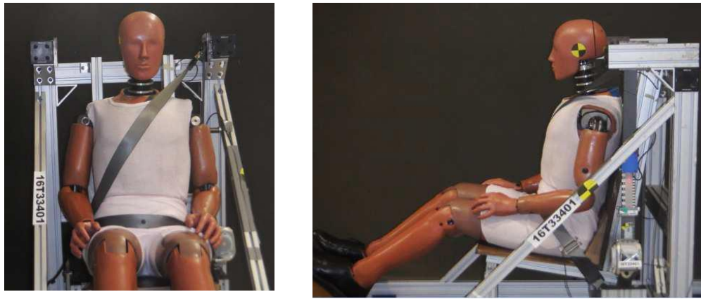
Figure 44: Retractor Pretensioner Deployment Test
