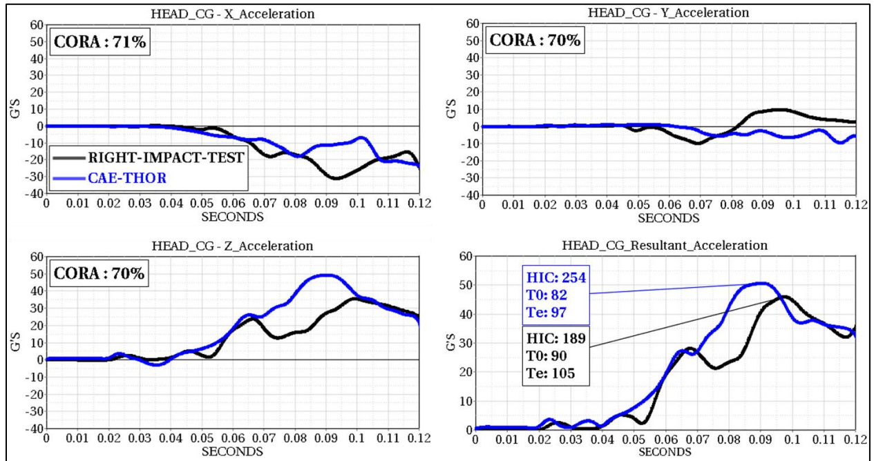
Figure 66: Passenger Head CG Acceleration
