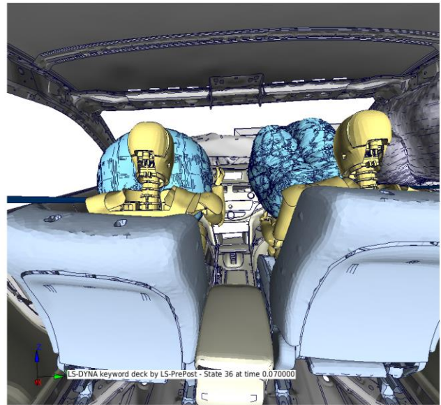
Figure 62: Test Versus CAE at 70 ms
