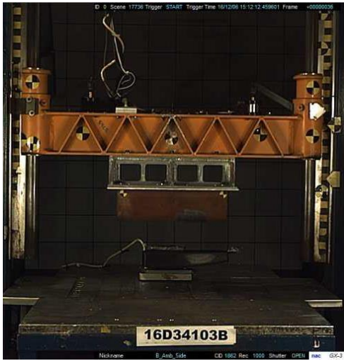
Figure 36: Side Air Bag Drop Tower Test Setup and FEA Model Setup
