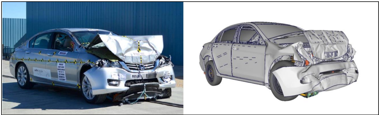
Figure 2: Test Versus CAE Model – Post-Crash Comparison
