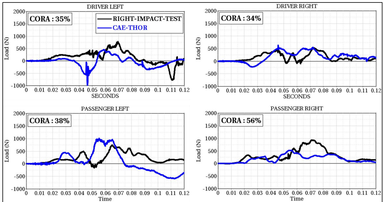
Figure 70: Driver and Passenger Femur Force
