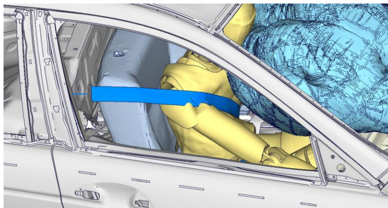
Figure 56: Seat belt slip in between shoulder and arm joint
