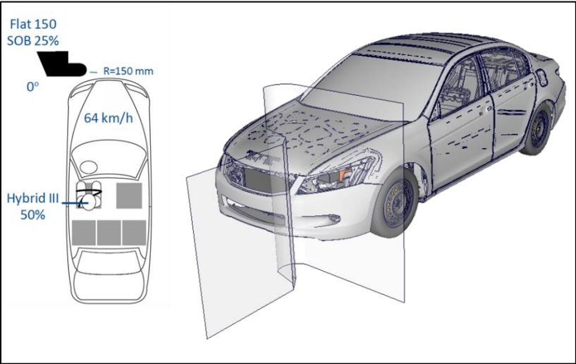
Figure 8: IIHS Small Overlap Test – Test Setup
