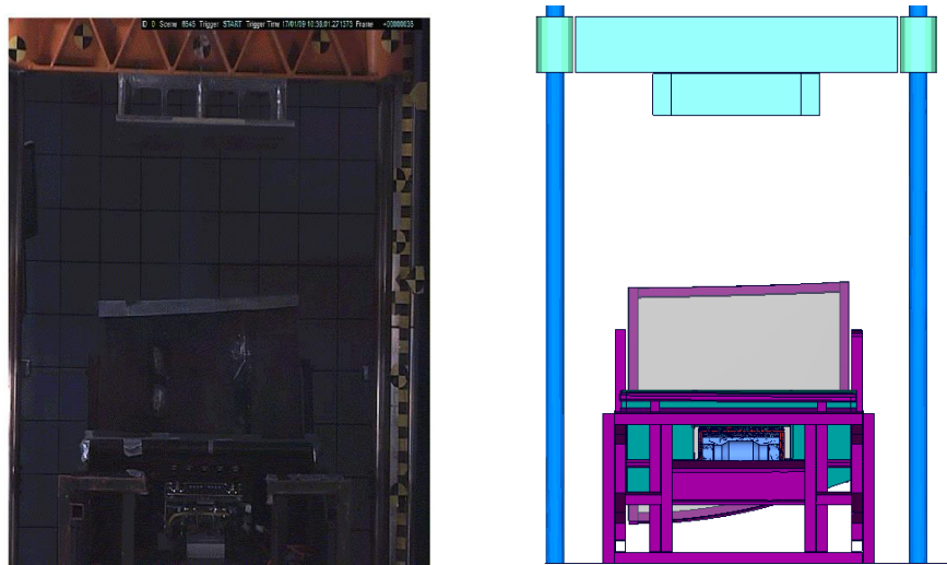
Figure 33: Passenger Air Bag Drop Tower Test Setup and FEA Model Setup
