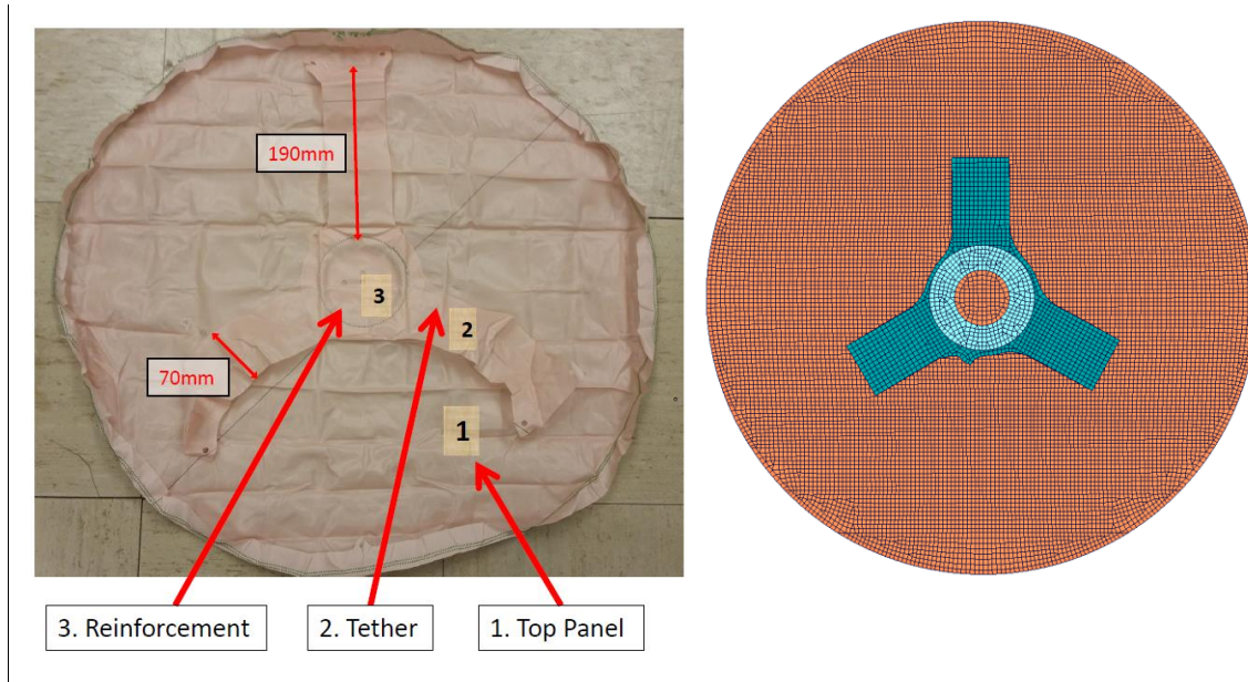
Figure 27: Drive Air Bag FE Model Before Folding
