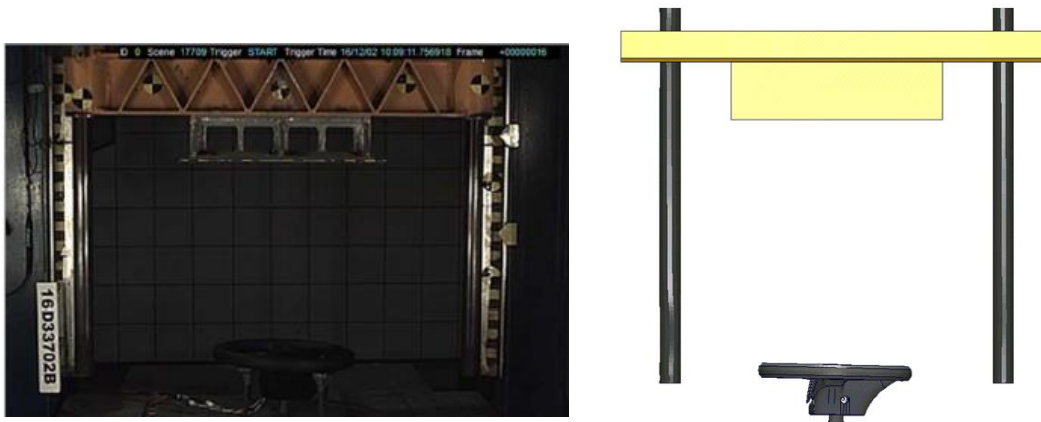
Figure 29: Drive Air Bag Drop Tower Test Setup and FEA Model Setup
