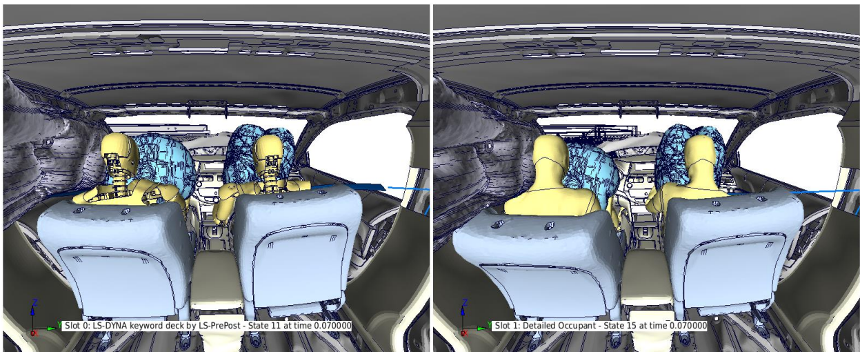
Figure 74: CAE-THOR Versus GHBMC at 70 ms
