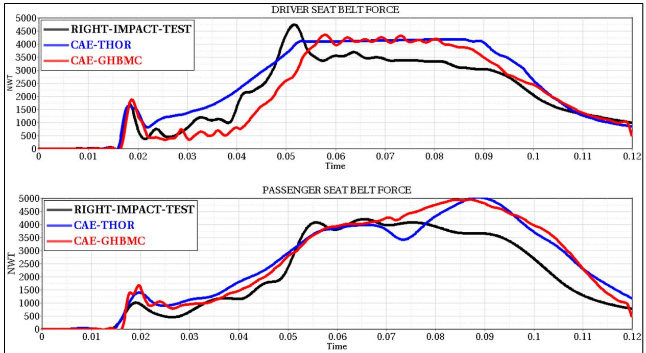
Figure 92: Driver and Passenger Seat belt Force
