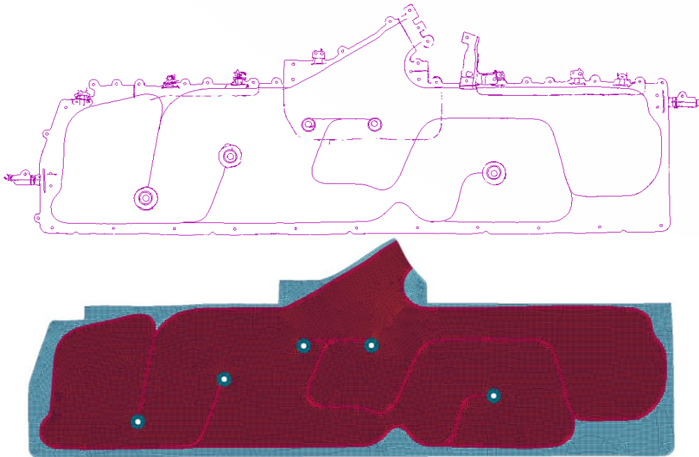
Figure 38: Side Curtain Air Bag FE Model before Folding
