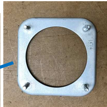
1. Insert retainer into inflator opening and secure with studs
