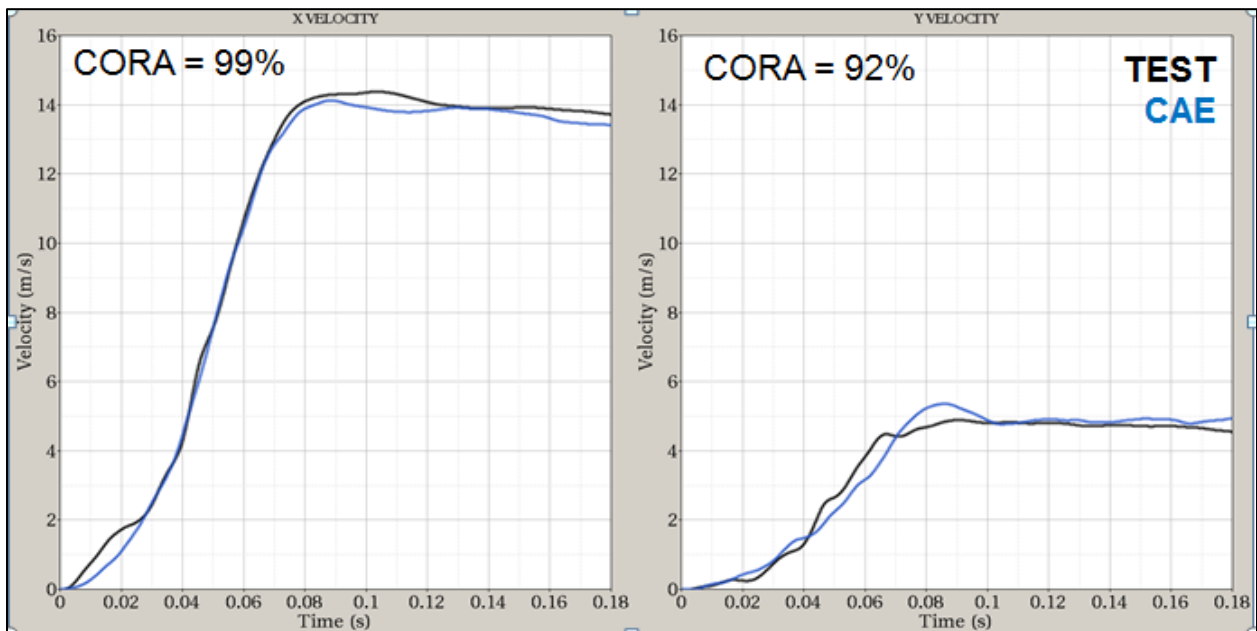
Figure 16: Test Versus CAE X and Y Velocity
