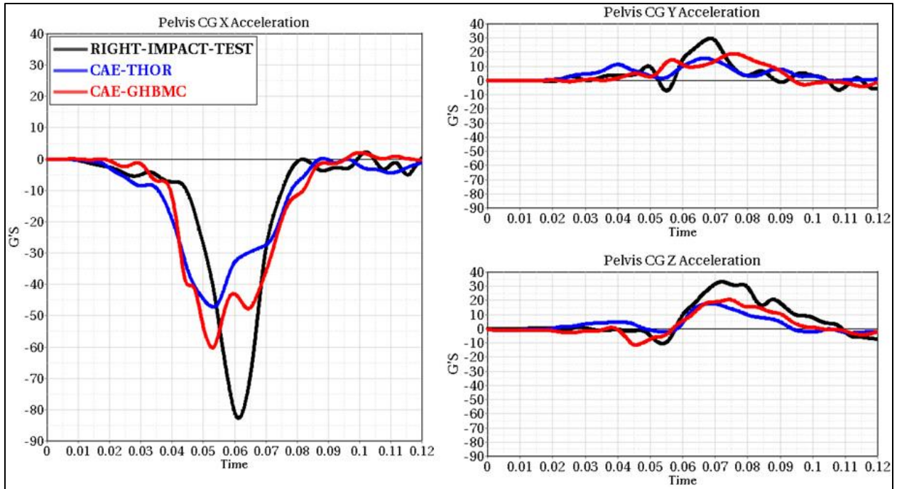
Figure 90: Driver Pelvic CG Acceleration
