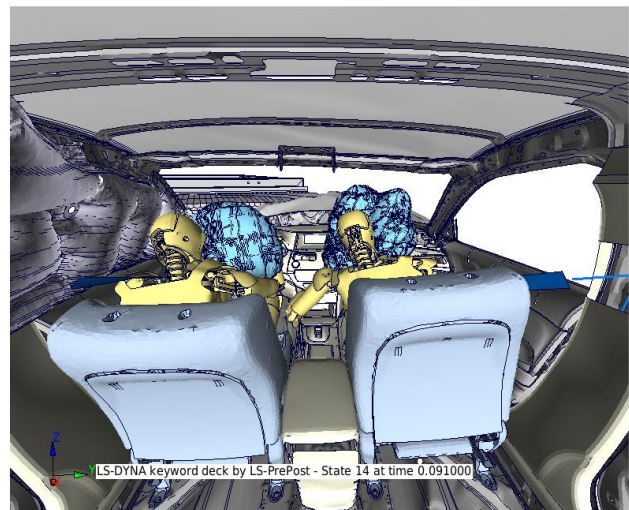
Figure 50: Test Versus CAE at 90 ms
