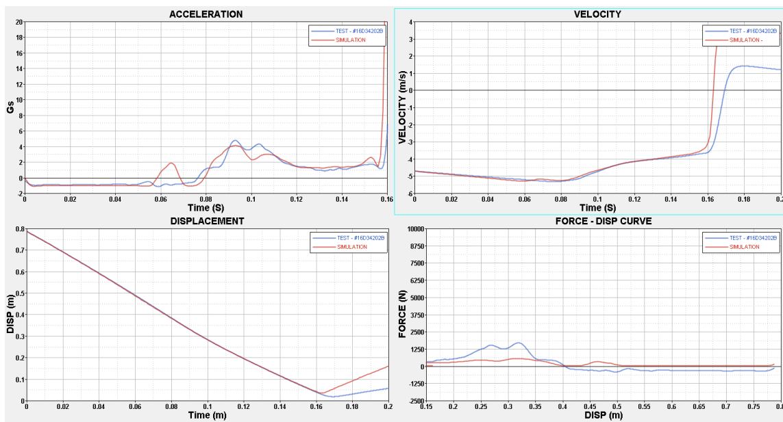
Figure 34: Passenger Air Bag Validation – Drop Tower Test and Simulation
