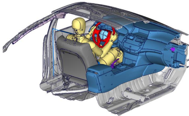
Figure 45: Sled Model Setup
