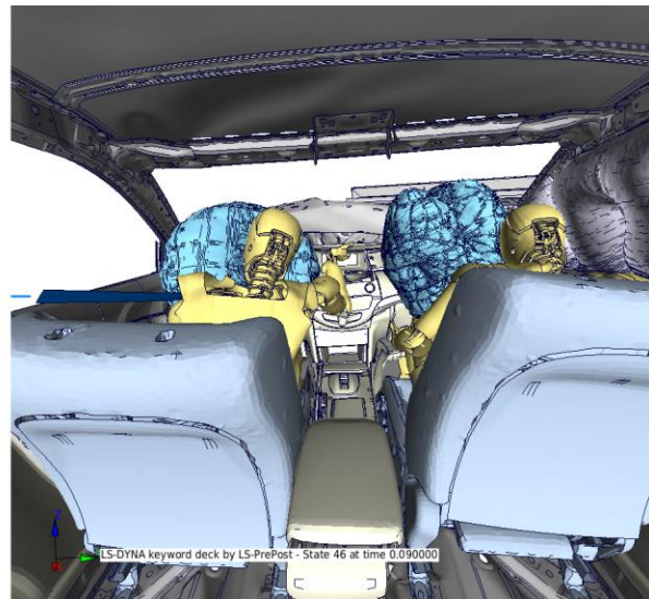
Figure 63: Test Versus CAE at 90 ms
