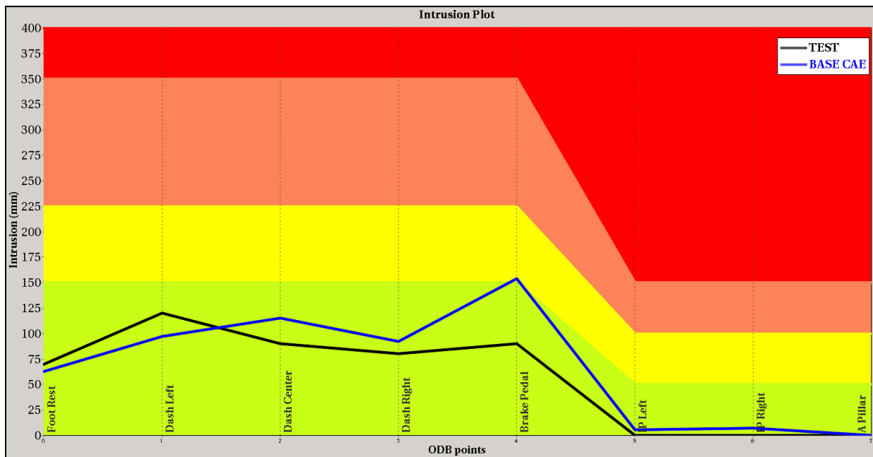
Figure 7: IIHS Frontal Moderate – Intrusion Values Comparison Test Versus CAE Results for Baseline
