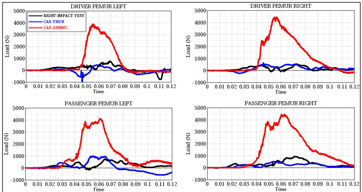
Figure 93: Driver and Passenger Femur Force
