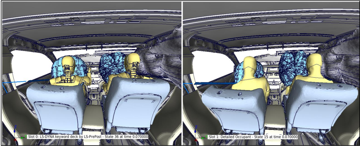
Figure 85: THOR CAE Versus GHBMC Model at 70 ms
