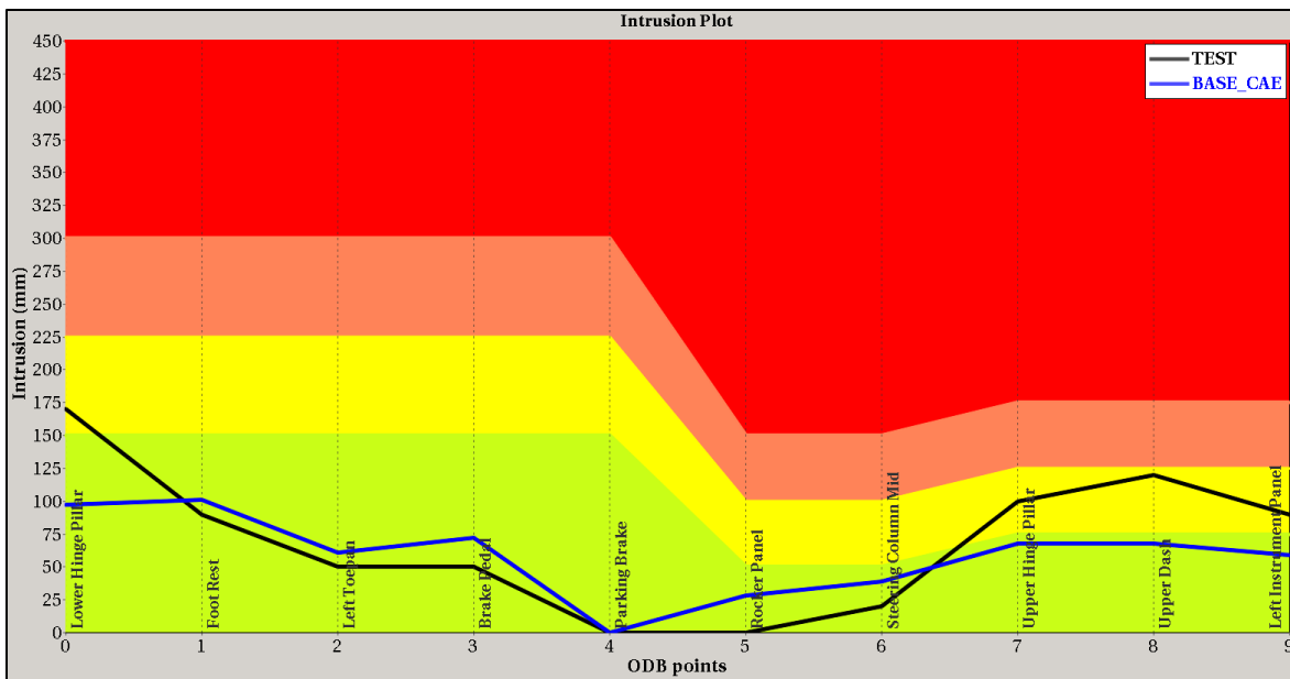
Figure 11: IIHS Small Overlap Intrusion - Test Versus Base CAE
