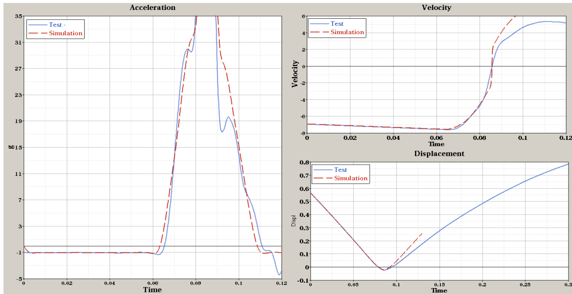
Figure 41: Side Curtain Air Bag Validation – Drop Tower Test and Simulation
