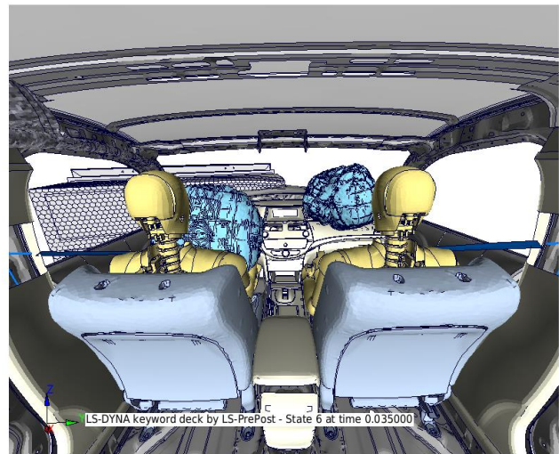
Figure 48: Test Versus CAE at 35 ms
