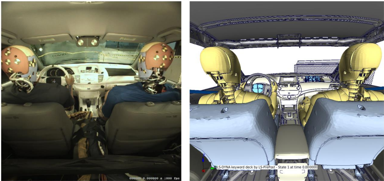
Figure 60: Test Versus CAE at 0 ms
