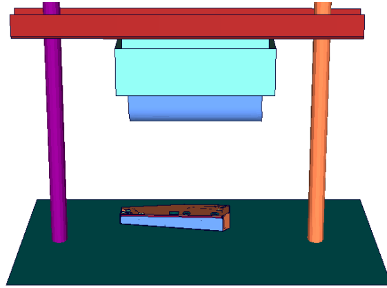
Figure 36: Side Air Bag Drop Tower Test Setup and FEA Model Setup
