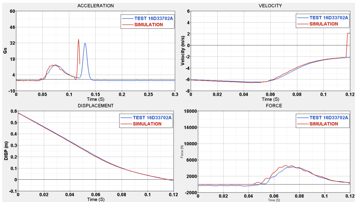
Figure 30: Drive Air Bag Validation – Drop Tower Test and Simulation
