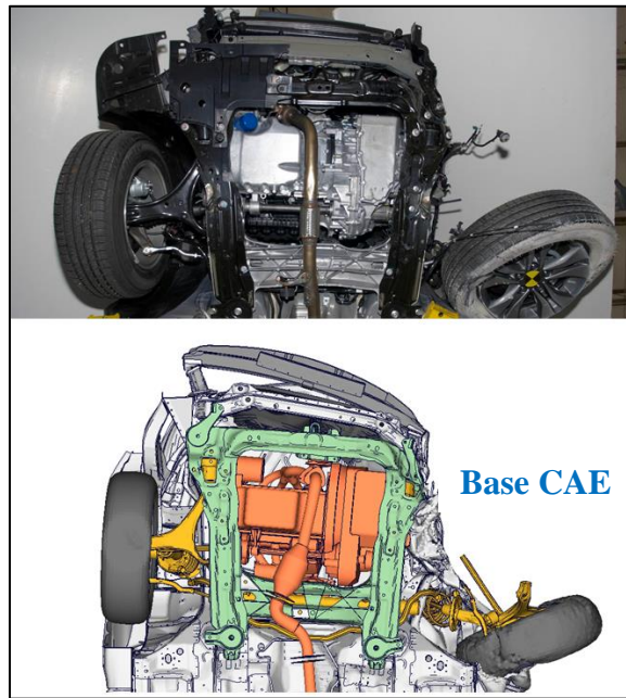
Figure 10: IIHS Small Overlap Test Versus Base CAE
