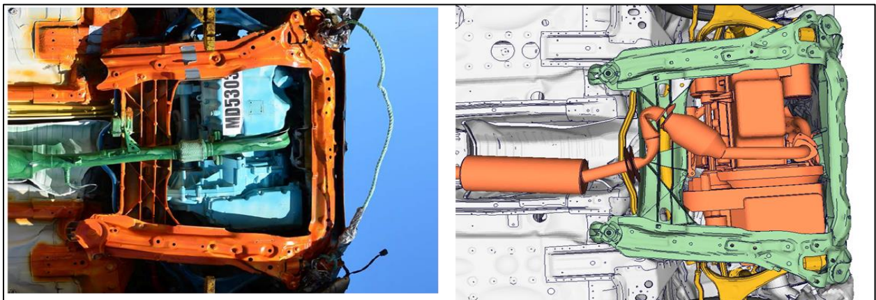
Figure 3: Test Versus CAE Model – Post-Crash Comparison
