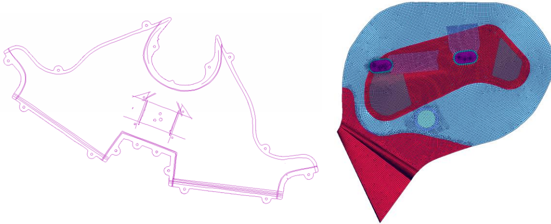
Figure 31: Passenger Air Bag – 2D Geometry and Flattened FE Bag
