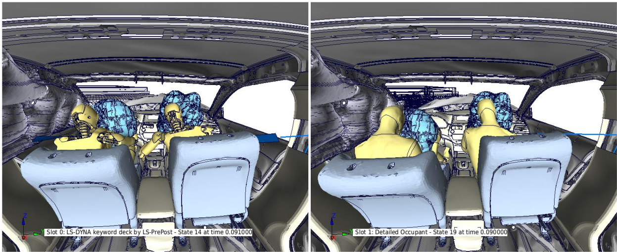
Figure 75: CAE-THOR Versus GHBMC at 90 ms
