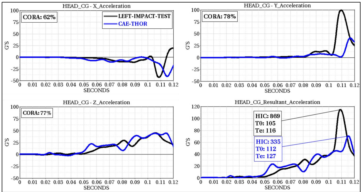
Figure 53: Passenger Head CG Acceleration
