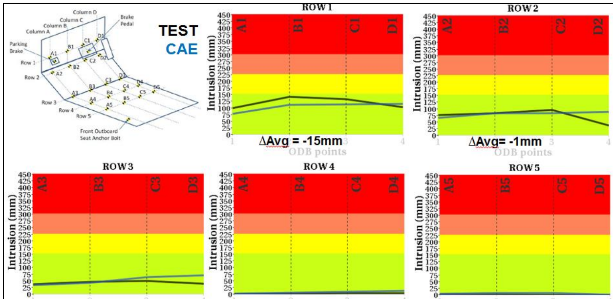
Figure 18: Test Versus CAE NCAP Driver Floor Pan Intrusion
