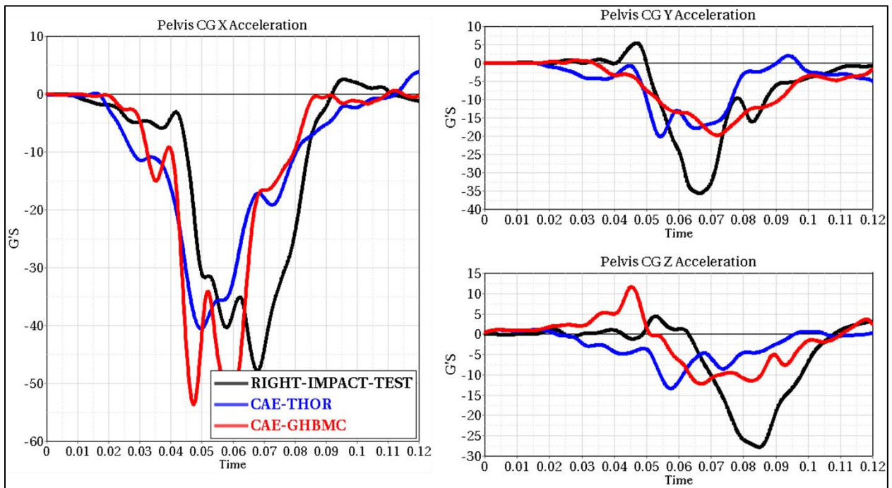
Figure 91: Passenger Pelvic CG Acceleration
