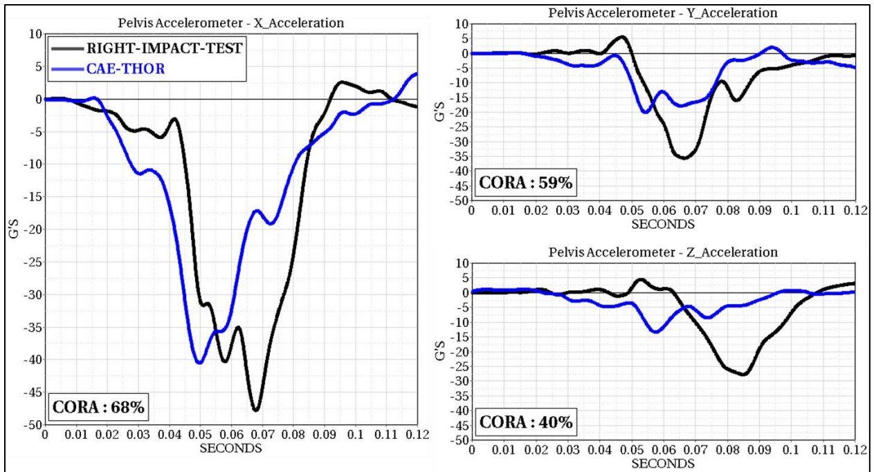
Figure 68: Passenger Pelvic CG Acceleration
