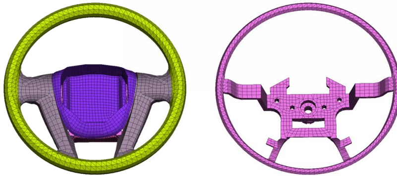
Figure 20: Steering Wheel
