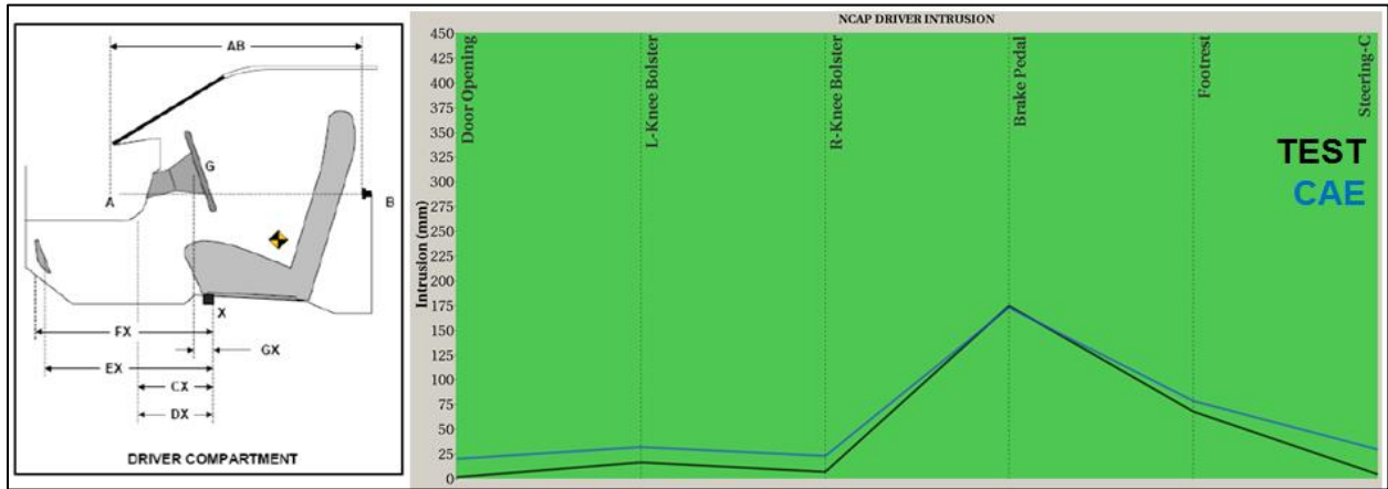
Figure 17: Test Versus CAE NCAP Driver Compartment Intrusion
