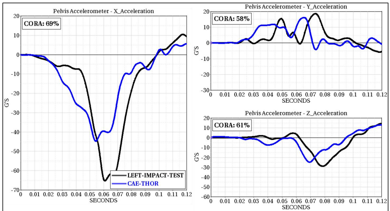
Figure 55: Passenger Pelvic CG Acceleration
