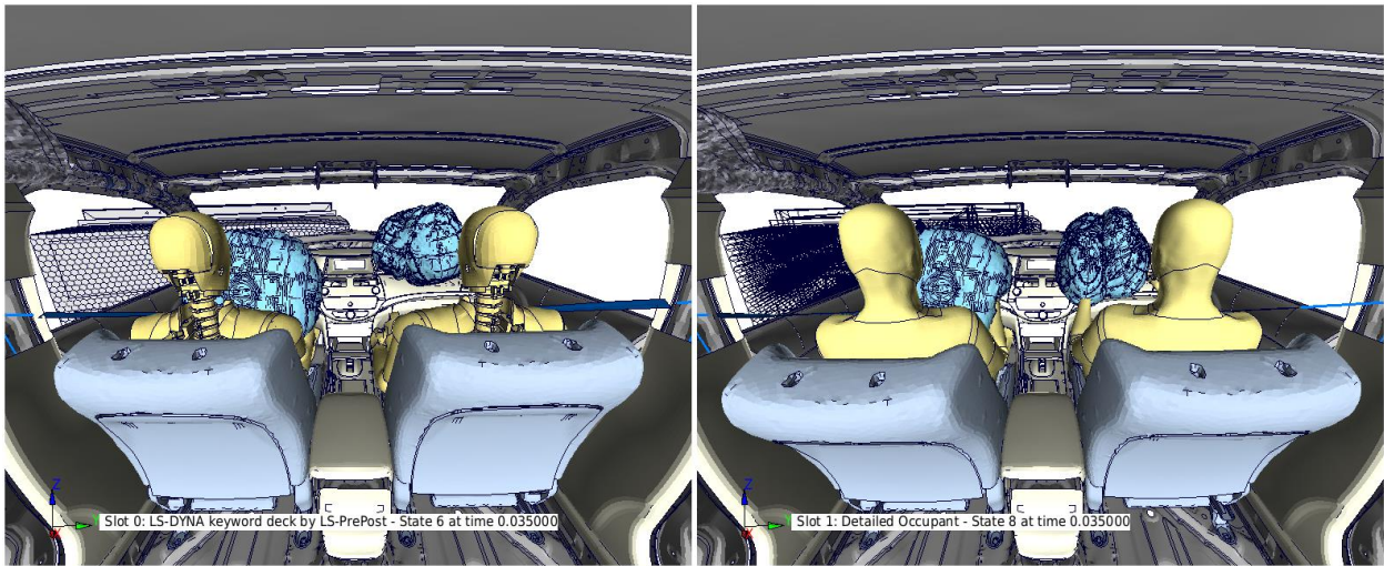
Figure 73: CAE-THOR Versus GHBMC at 35 ms
