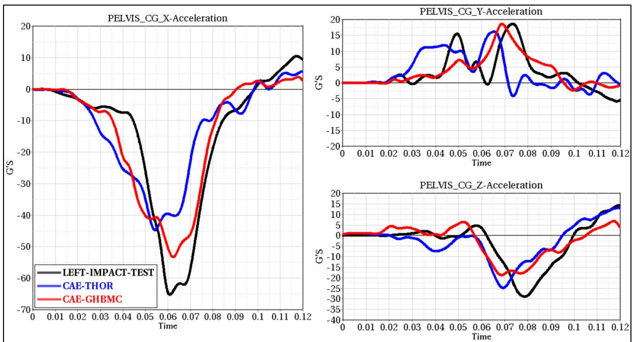
Figure 80: Passenger Pelvic CG Acceleration
