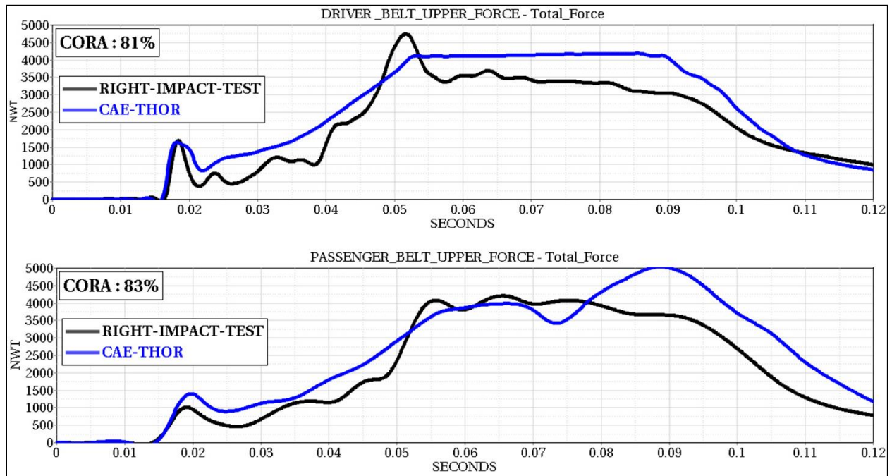
Figure 69: Driver and Passenger Seat belt Force
