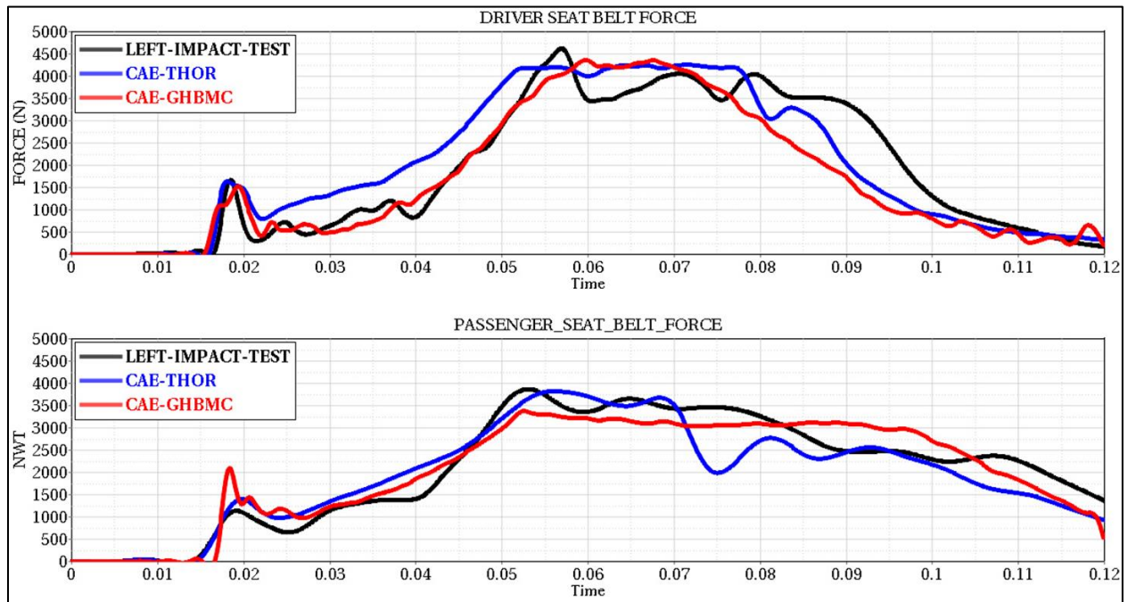
Figure 81: Driver and Passenger Belt Force
