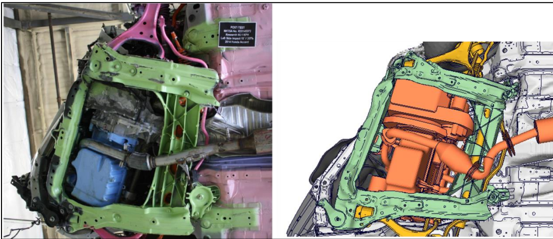
Figure 14: NHTSA Oblique Test Left – Post-Crash Comparison Test Versus CAE Baseline
