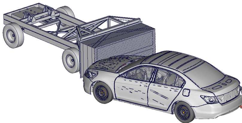
Figure 59: Right Oblique Impact Setup
