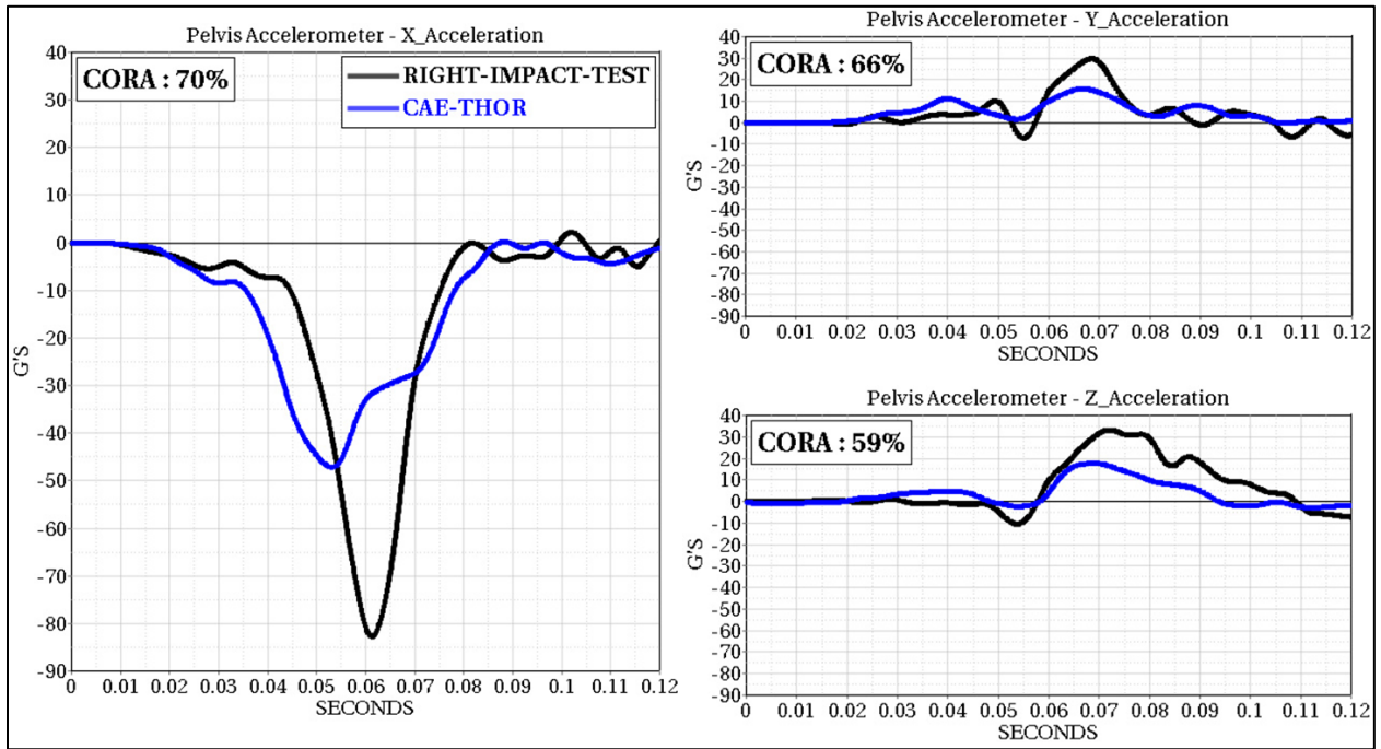
Figure 67: Driver Pelvic CG Acceleration
