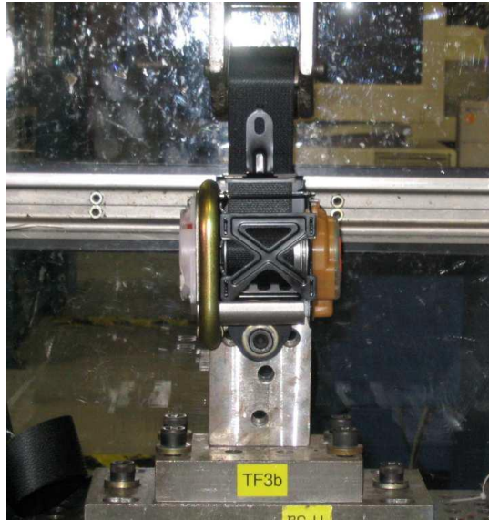
Figure 43: Retractor Pay-out (load limiter) Test Setup
