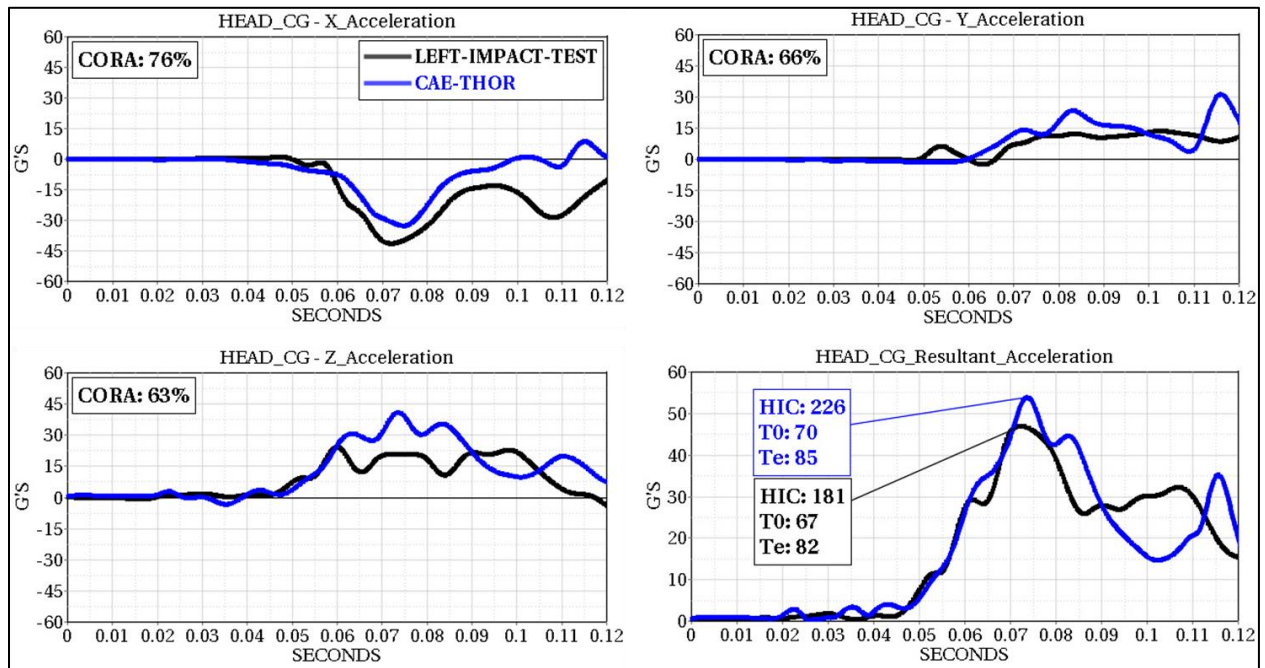
Figure 52: Driver Head CG Acceleration
