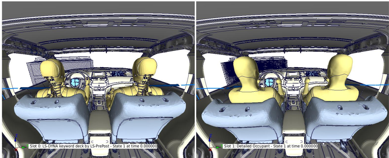
Figure 72: CAE-THOR Versus GHBM at 0 ms
