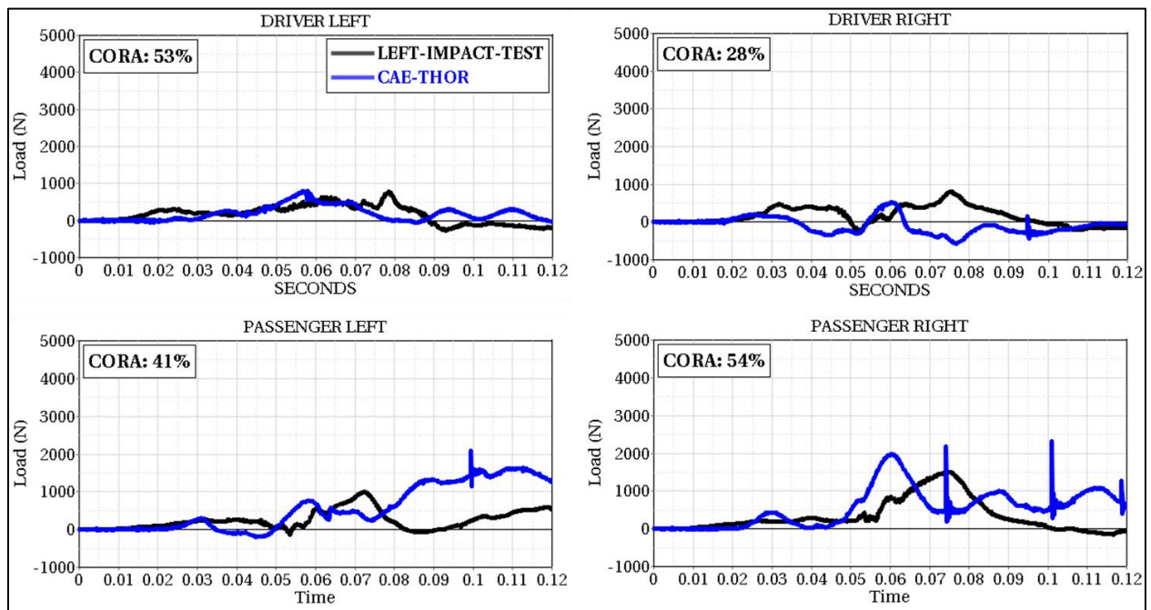
Figure 58: Driver and Passenger Femur Force
