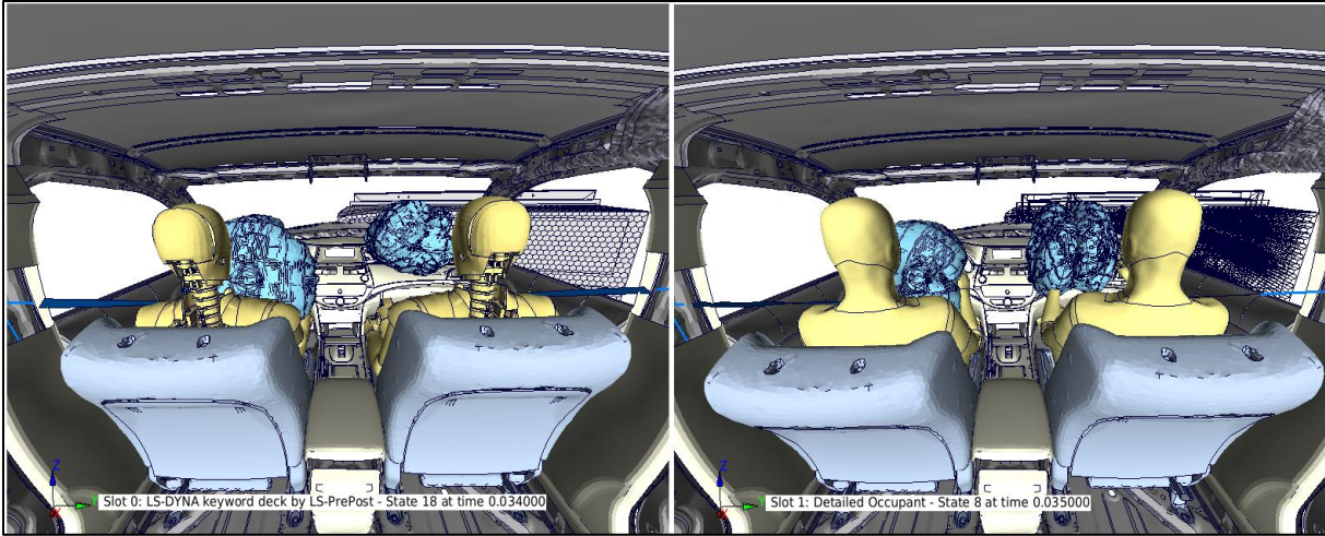
Figure 84: THOR CAE Versus GHBMC Model at 35 ms
