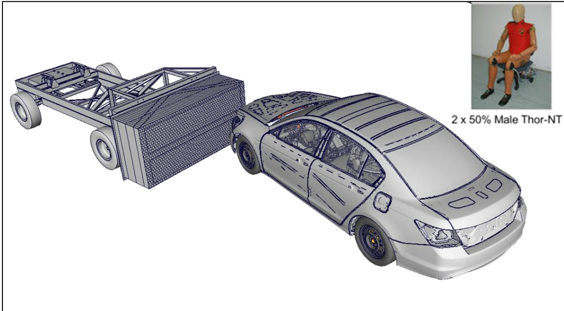
Figure 12: NHTSA Oblique Test Left
