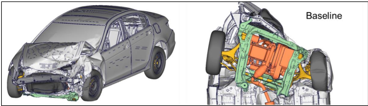
Figure 6: IIHS Frontal Offset - Post-Crash CAE Results for Baseline
