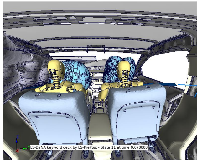
Figure 49: Test Versus CAE at 70 ms
