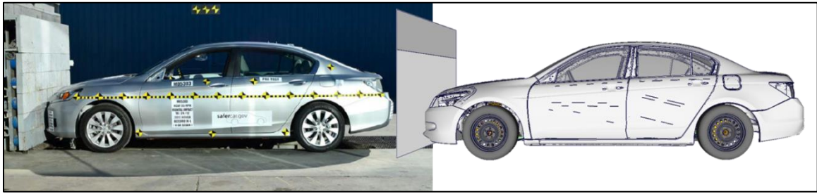
Figure 1: Test Versus CAE Model – NCAP Frontal Test Setup
