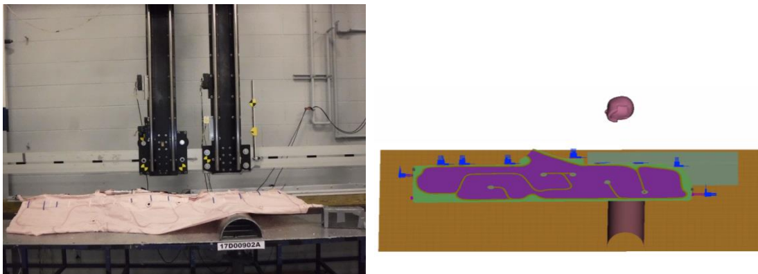
Figure 40: Side Curtain Air Bag Drop Tower Test Setup and FEA Model Setup
