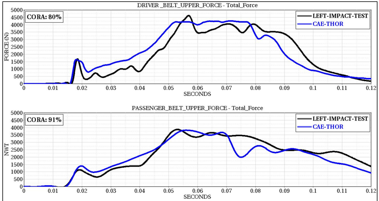
Figure 57: Driver and Passenger Seat belt Force
