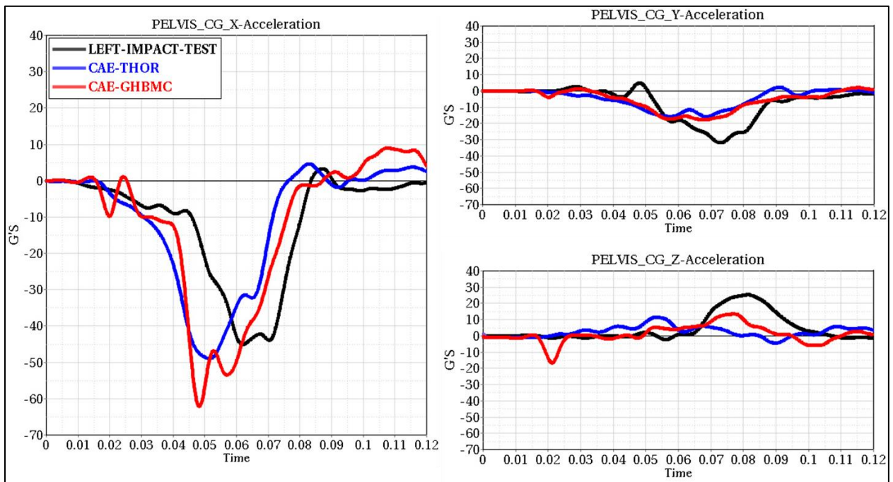
Figure 79: Driver Pelvic CG Acceleration
