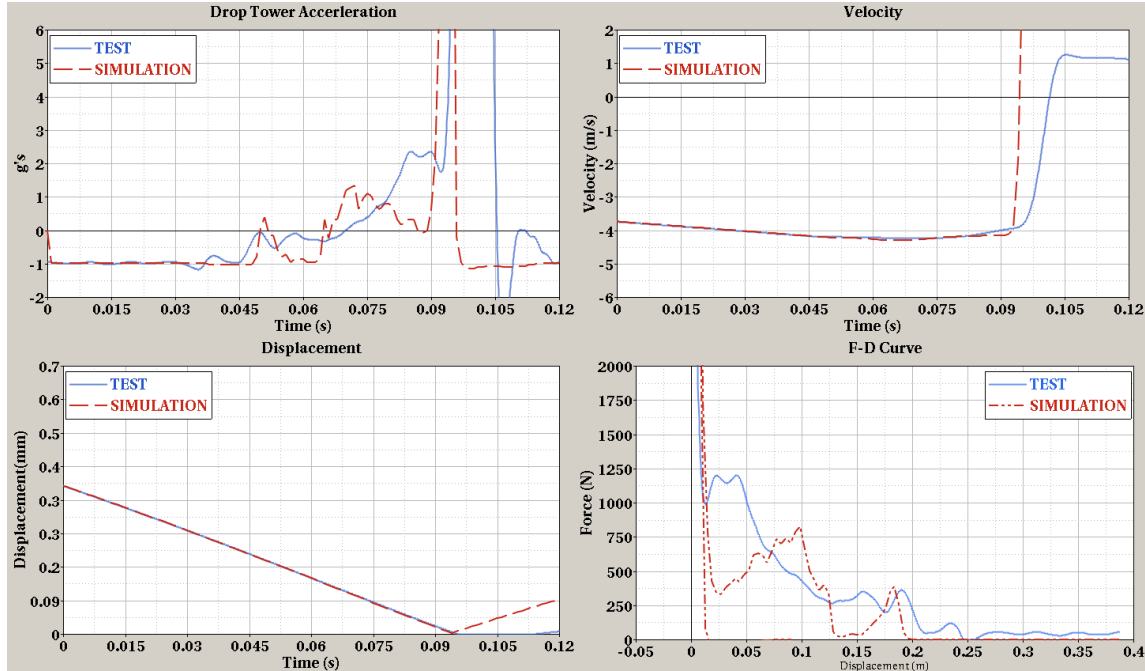
Figure 37: Side Air Bag Validation – Drop Tower Test and Simulation
