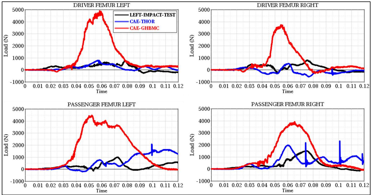
Figure 82: Driver and Passenger Femur Force
