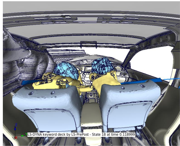
Figure 51: Test Versus CAE at 120 ms
