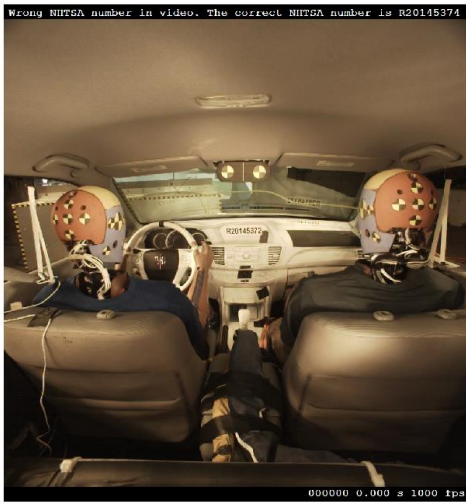
Figure 47: Test Versus CAE at 0 ms
