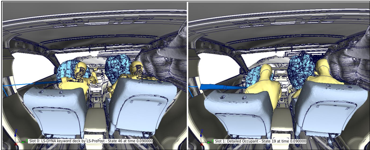
Figure 86: THOR CAE Versus GHBM Model at 90 ms
