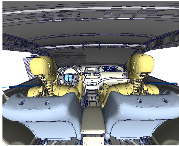
Figure 47: Test Versus CAE at 0 ms
