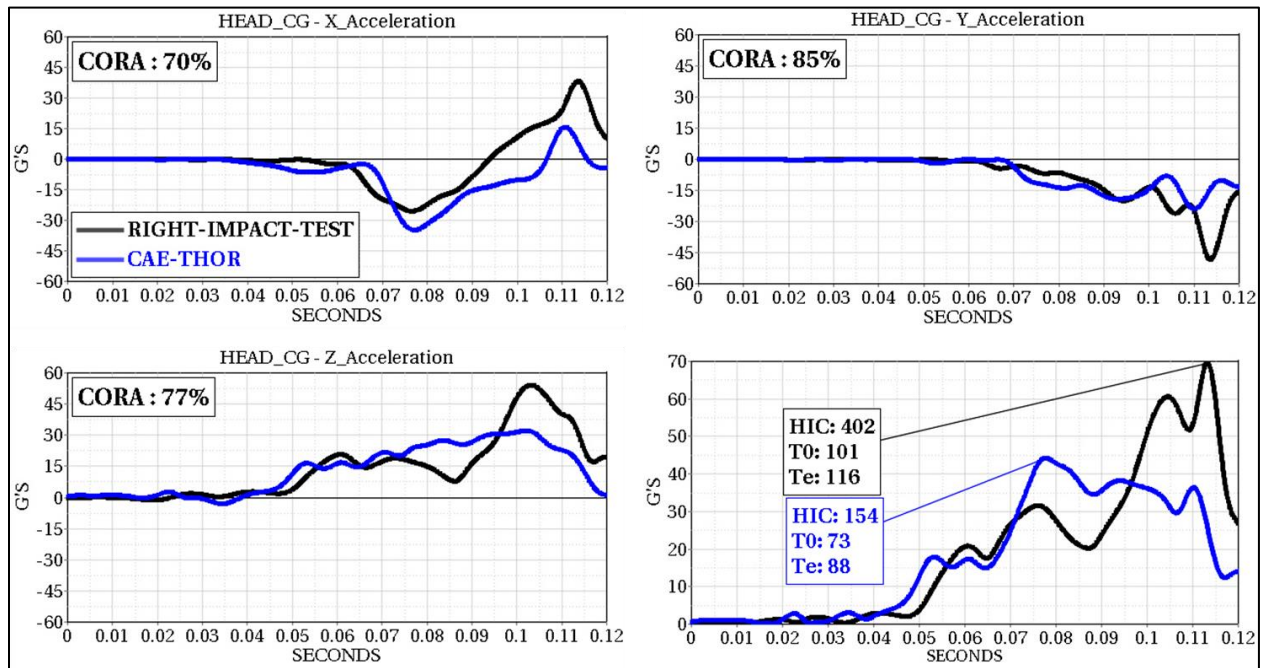
Figure 65: Driver Head CG Acceleration
