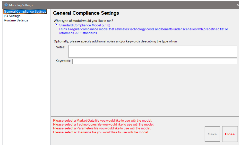
Figure 30. Select Standard Compliance Model
