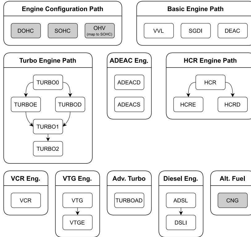
Figure 2. Engine-Level Paths
